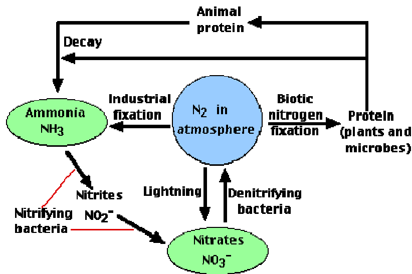
Figure 6: The Nitrogen Cycle
